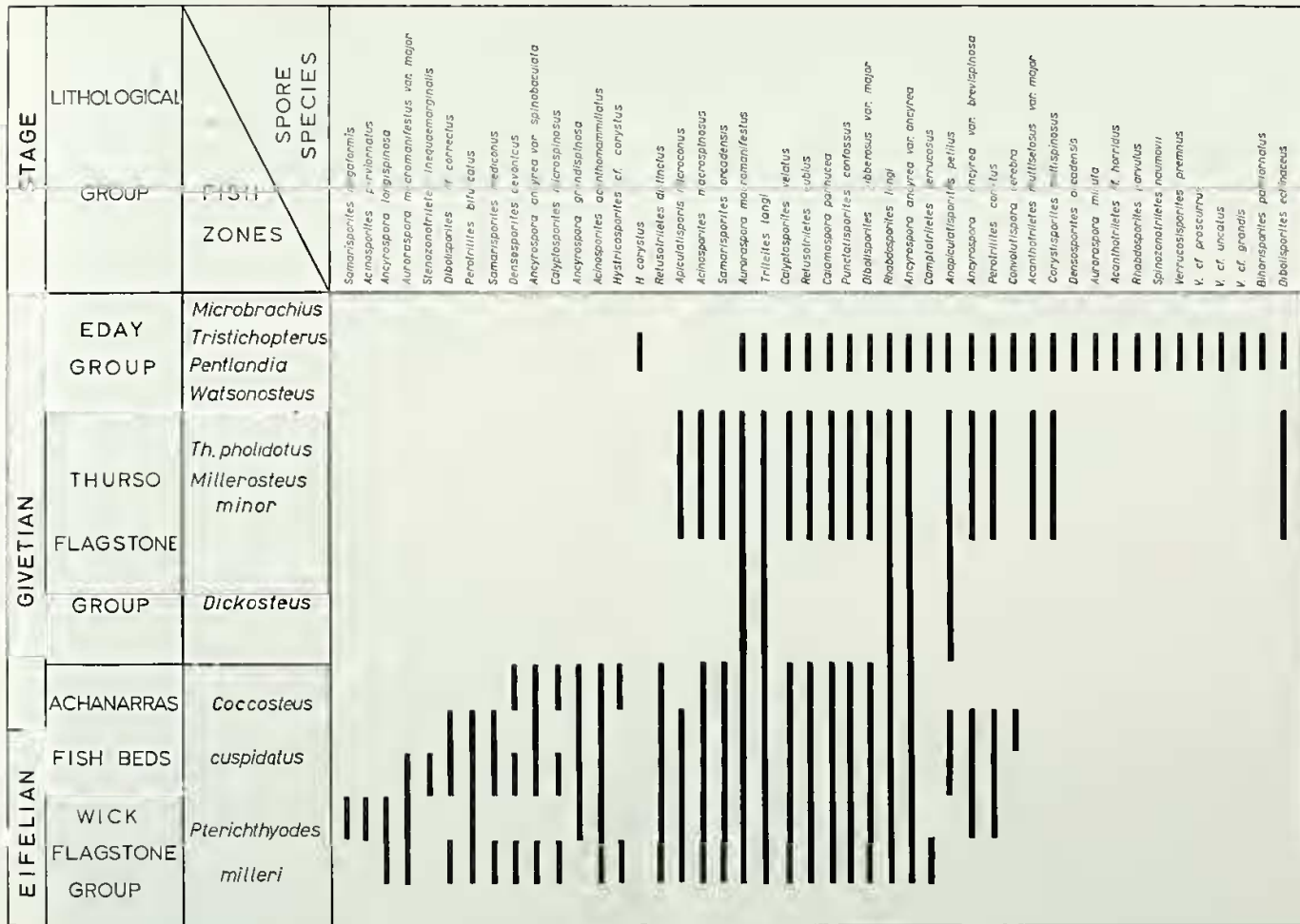
TEXT-FIG. 9. Range chart showing spore distribution in the Middle Old Red Sandstone of the Orcadian basin.
